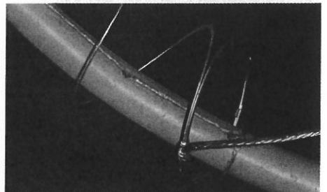
PHOTO 2: Detail of how the Slinky is mounted on the water pipe. The string is tied to the Slinky on the hidden side of the pipe.
