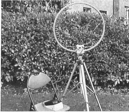
PHOTO 1: The completed Slinky loop antenna, mounted on a tripod.
