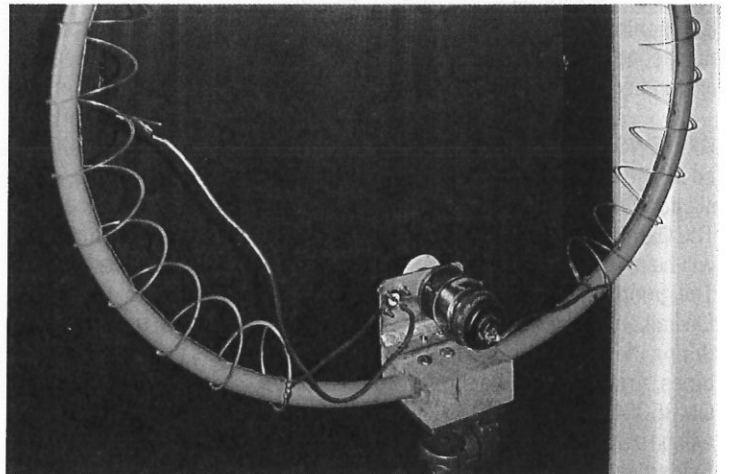
PHOTO 3: General view of the business end of the loop, showing the mounting block, capacitor/input socket bracket, wiring and my tapping point.
