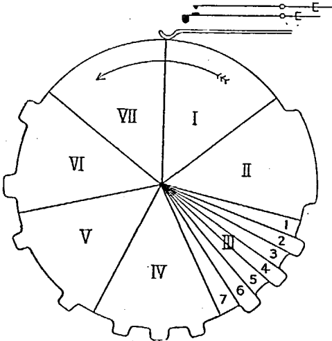
Fig. 3.—Diagram of cam disc for producing a letter E impulse train
