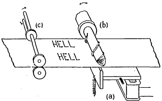
Fig. 4.—Diagram of receiving mechanism
