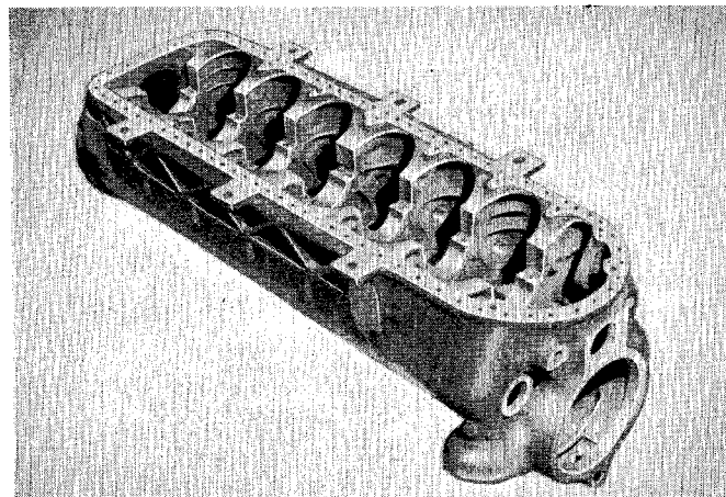
CRANKCASE OF AN AIRPLANE ENGINE, CAST IN A MAGNESIUM ALLOY
