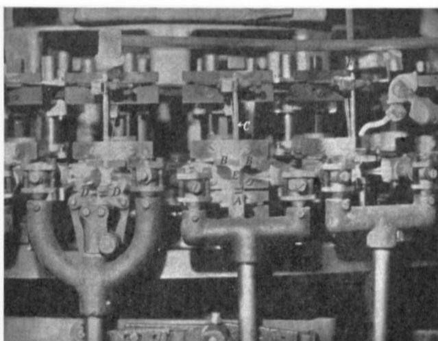
Fig. 5. Pinch-making machine
