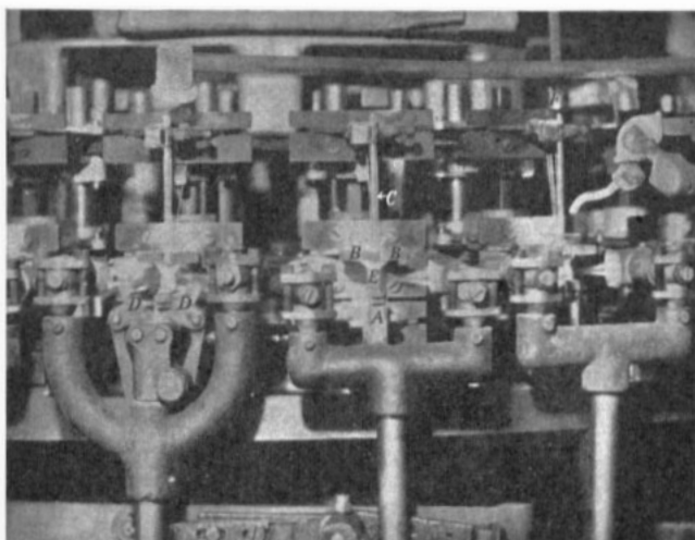
Fig. 5. Pinch-making machine
