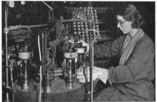
Fig. 7. Sealing-in machine
