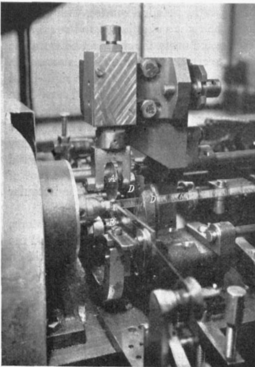
Fig. 2. Automatic grid notching machine
