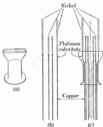
Fig. 4. Stages in the manufacture of the pinch or electrode support tube
