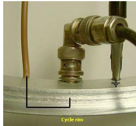
Hairpin coupling
