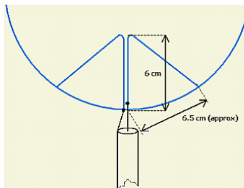
Quasi delta match.
